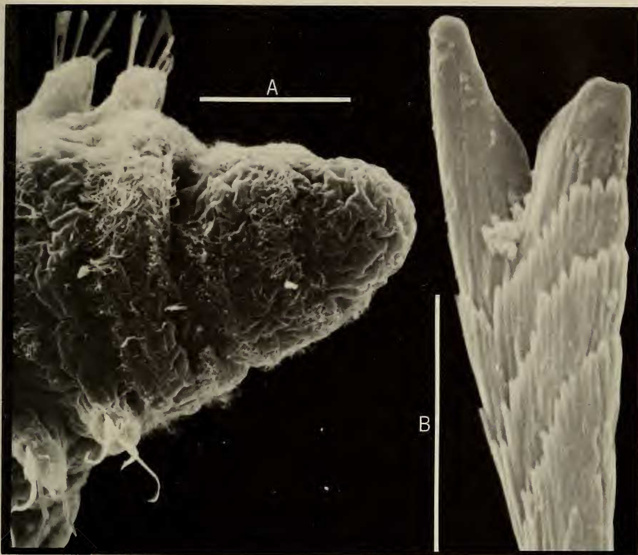
Fig. 2. Gymnodorvillea floridana , paratypes: A, Anterior region, dorsal view, showing ciliary bands, shrinkage due to fixation and/or critical-point drying; B, Furcate seta (SEM photomicrographs. Scales: A = 50 \mu\text{m} , B = 5 \mu\text{m} ).
